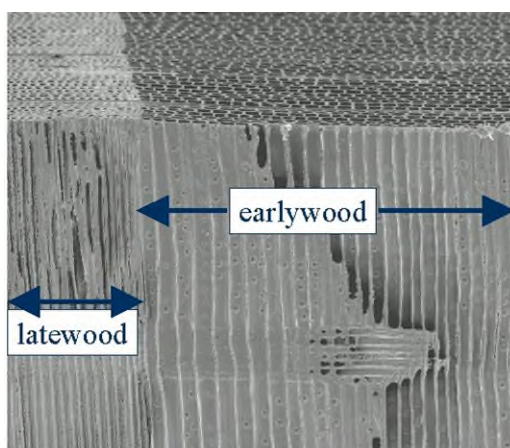
Figure 1: Scanning electron micrograph of a softwood
